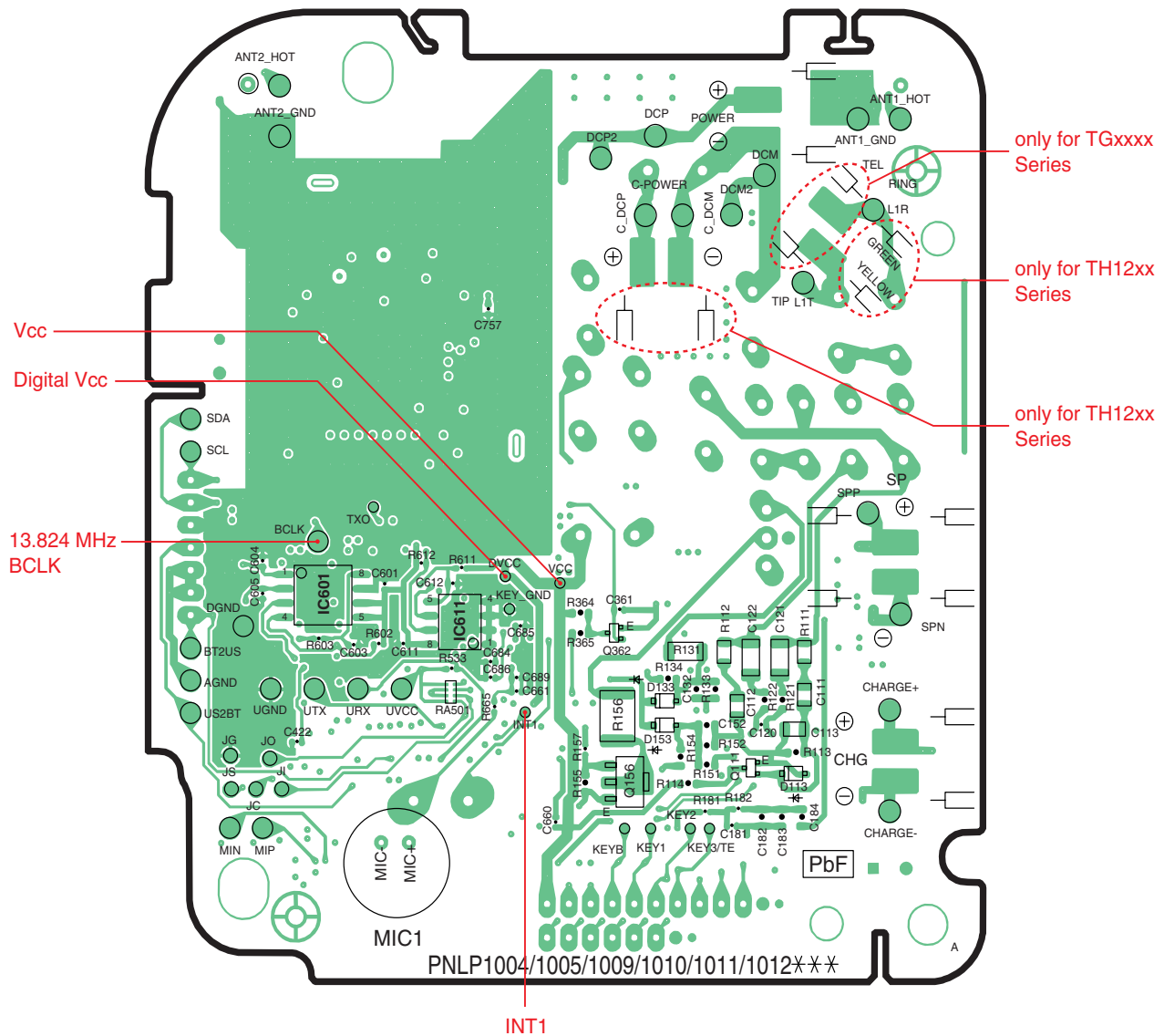
KX-TG9341/9342/9343/9344 CIRCUIT BOARD (Base Unit_Main (Bottom View))
