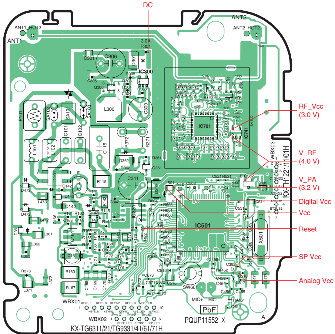
KX-TG9341/9342/9343/9344 CIRCUIT BOARD (Base Unit_Main (Component View))
